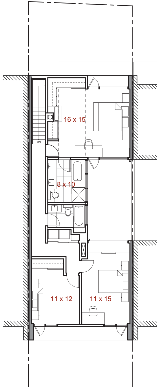
2ND FLOOR 948.91 SF
