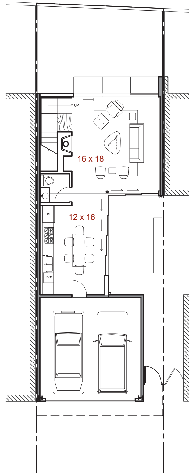
1ST FLOOR 582.90 SF GARAGE 334.56 SF
