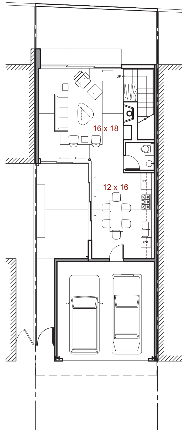
1ST FLOOR 582.90 SF GARAGE 334.56 SF
