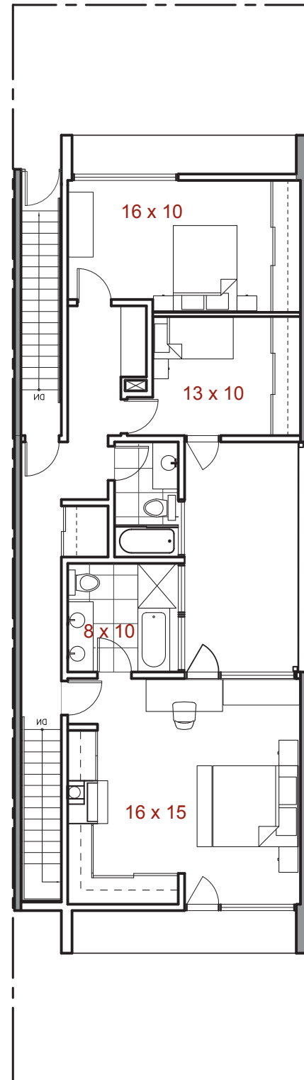
2ND FLOOR 1016.96 SF
