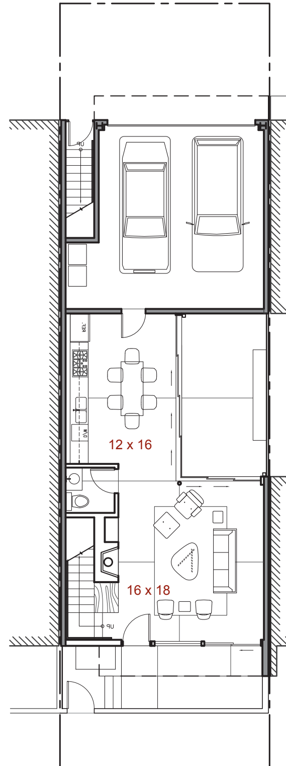
1ST FLOOR 585.19 SF GARAGE 393.36 SF
