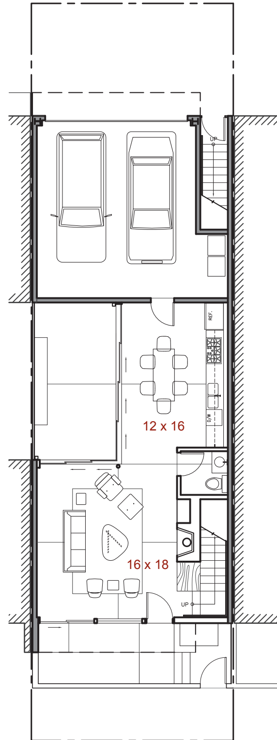
1ST FLOOR 585.19 SF GARAGE 393.36 SF
